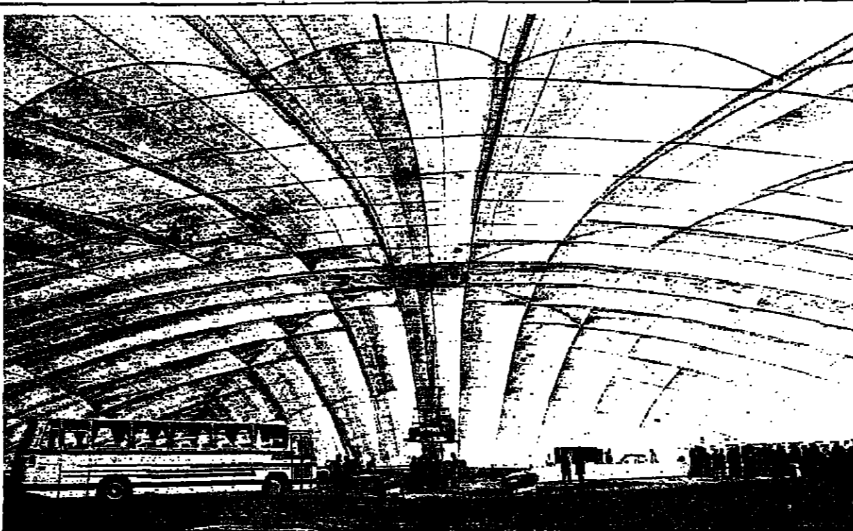
The widest-in-the-world inflatable structure set up near Paris represents a new concept for covering an area without pillars. It is constructed of a water- and air-tight material fixed to a cable running which is anchored on concrete blocks.
